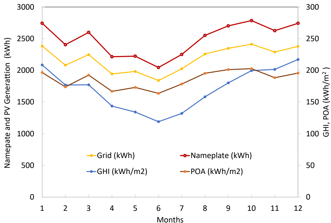
Figure 9: The expected energy production in relation the global horizontal and plane of array irradiances.
