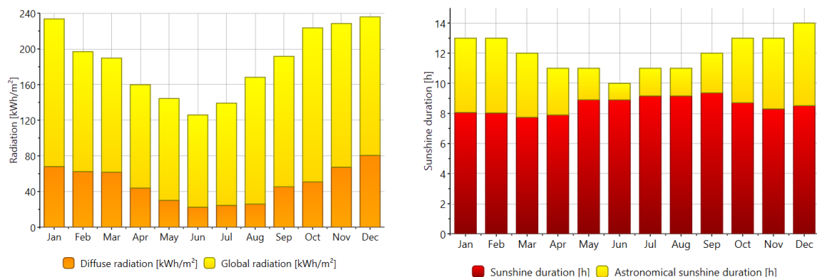
Figure 2: Global radiation data
